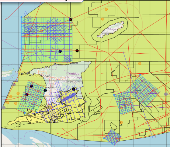
Seismic Viewer
