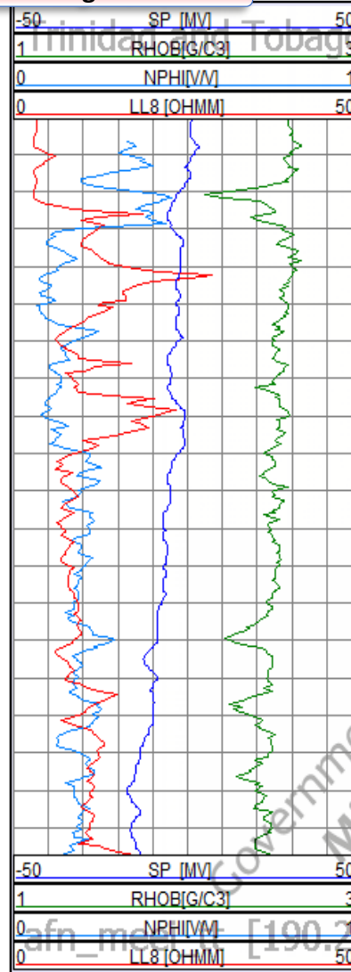
Log Viewer
